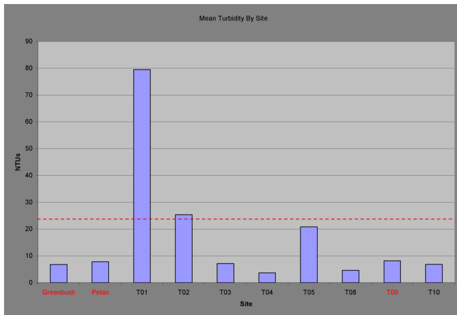
Graph 1 Mean Turbidity
